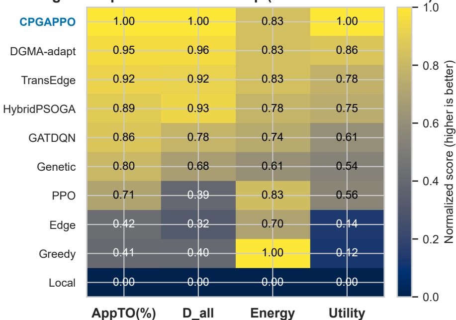
Algorithm performance heatmap (cross-DAG seed-mean)
